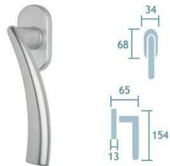
Manilla para ventana Ref. 772/DK/26D Nadir 2udes.
