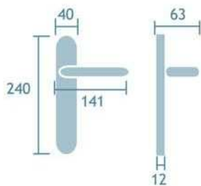
Manilla con placa Ref. 1030/SF/26D Link
